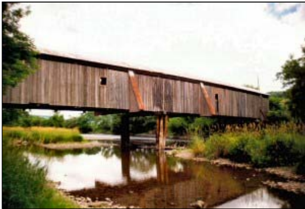
Hamden bridge before 2001
